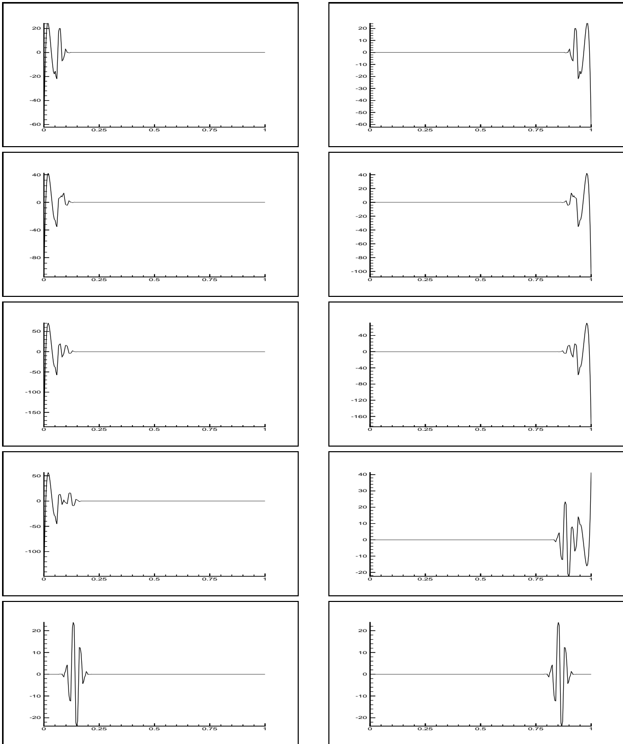
Figure 5.4.6: Dual wavelets \tilde{\psi}_{5,k} at left and right boundary.
