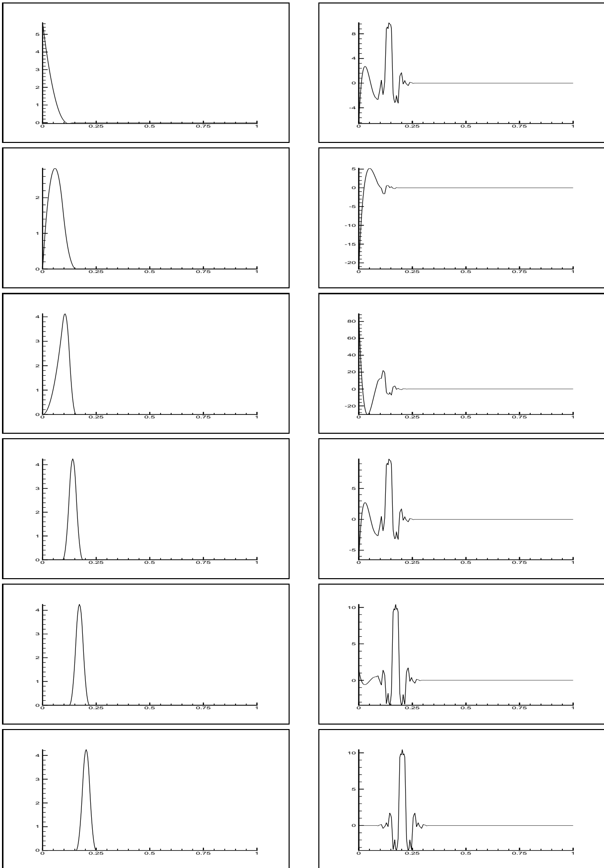
Figure 5.4.9: Primal and dual generators \phi_{5,k} for the Bernstein case.
