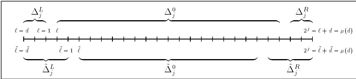
Figure 3.2.1: Index sets for the interval for d = 3 , \tilde{d} = 5 , \ell = 4 , \tilde{\ell} = \tilde{\ell}_2 = 6 .
