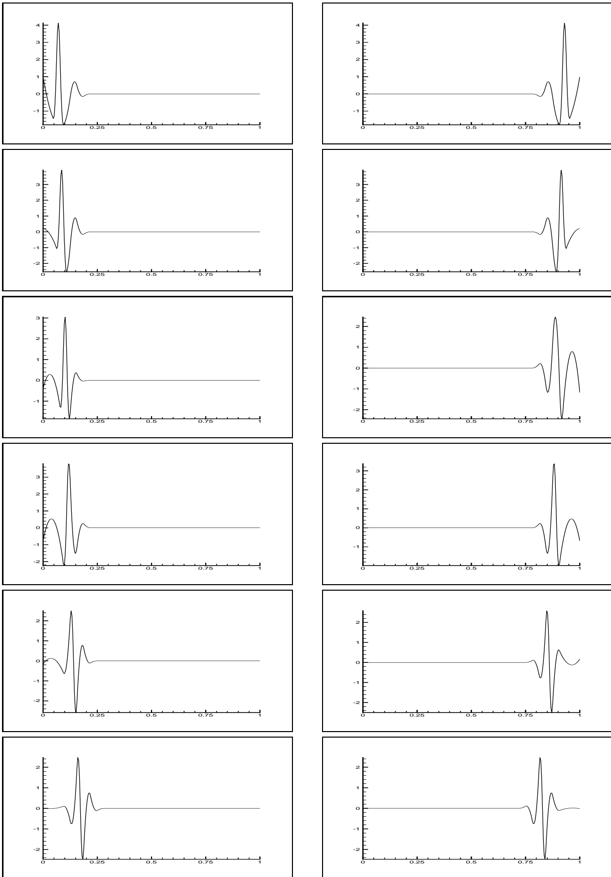
Figure 5.4.5: Primal wavelets \psi_{5,k} at left and right boundary.
