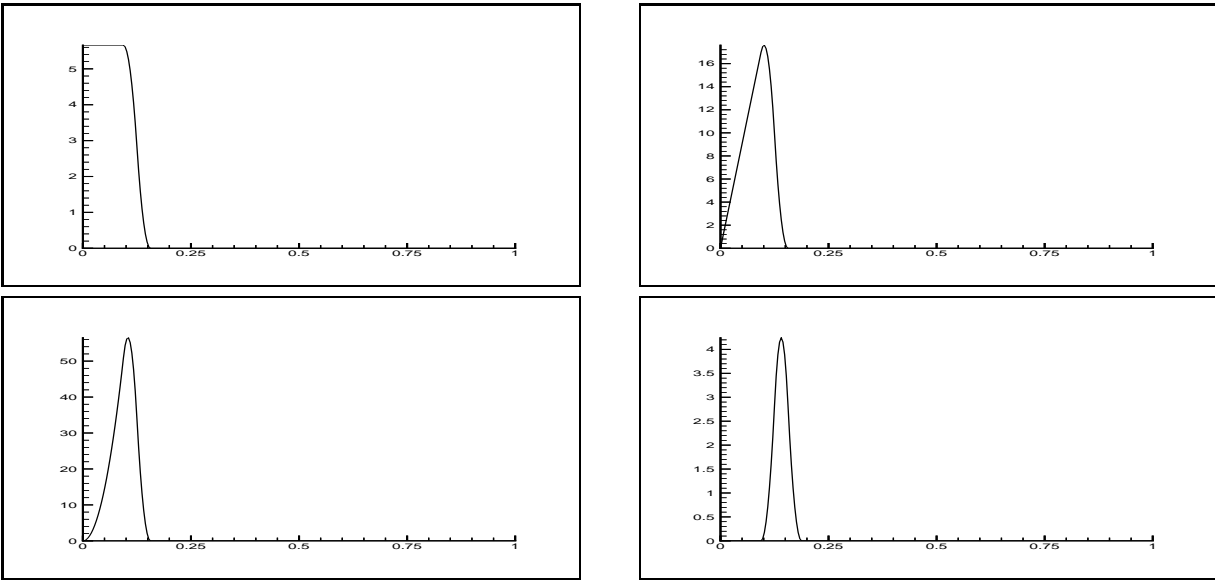
Figure 5.4.3: Primal generators \phi_{5,k} .
