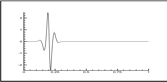
Figure 5.4.5: (continued) Primal wavelets \psi_{5,k} at left and right boundary.
