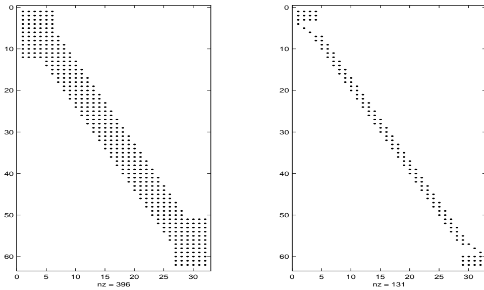
Figure 5.4.2: Nonzero pattern of refinement matrices M_{5,1}, \tilde{G}_{5,1}^T .
