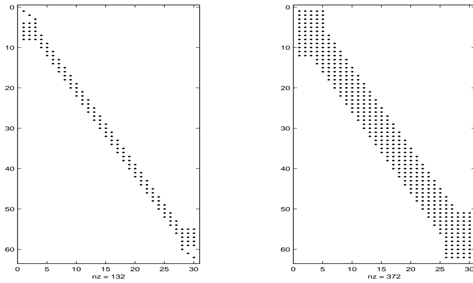
Figure 5.4.1: Nonzero pattern of refinement matrices M_{5,0}, \tilde{M}_{5,0} .
