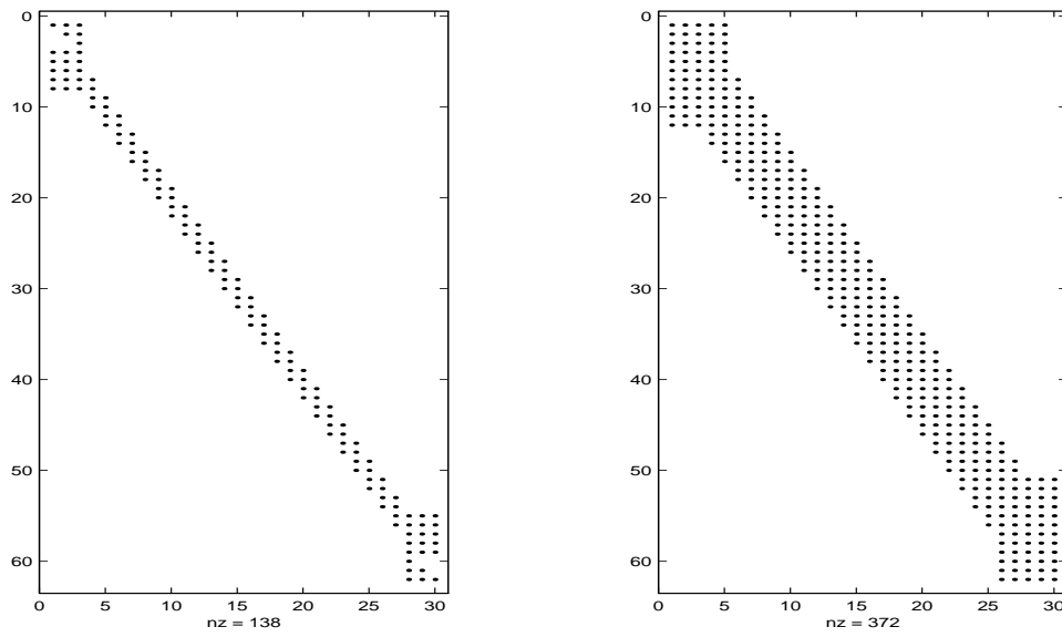
Figure 5.4.7: Nonzero pattern of refinement matrices \mathbf{M}_{5,0}, \tilde{\mathbf{M}}_{5,0} .
