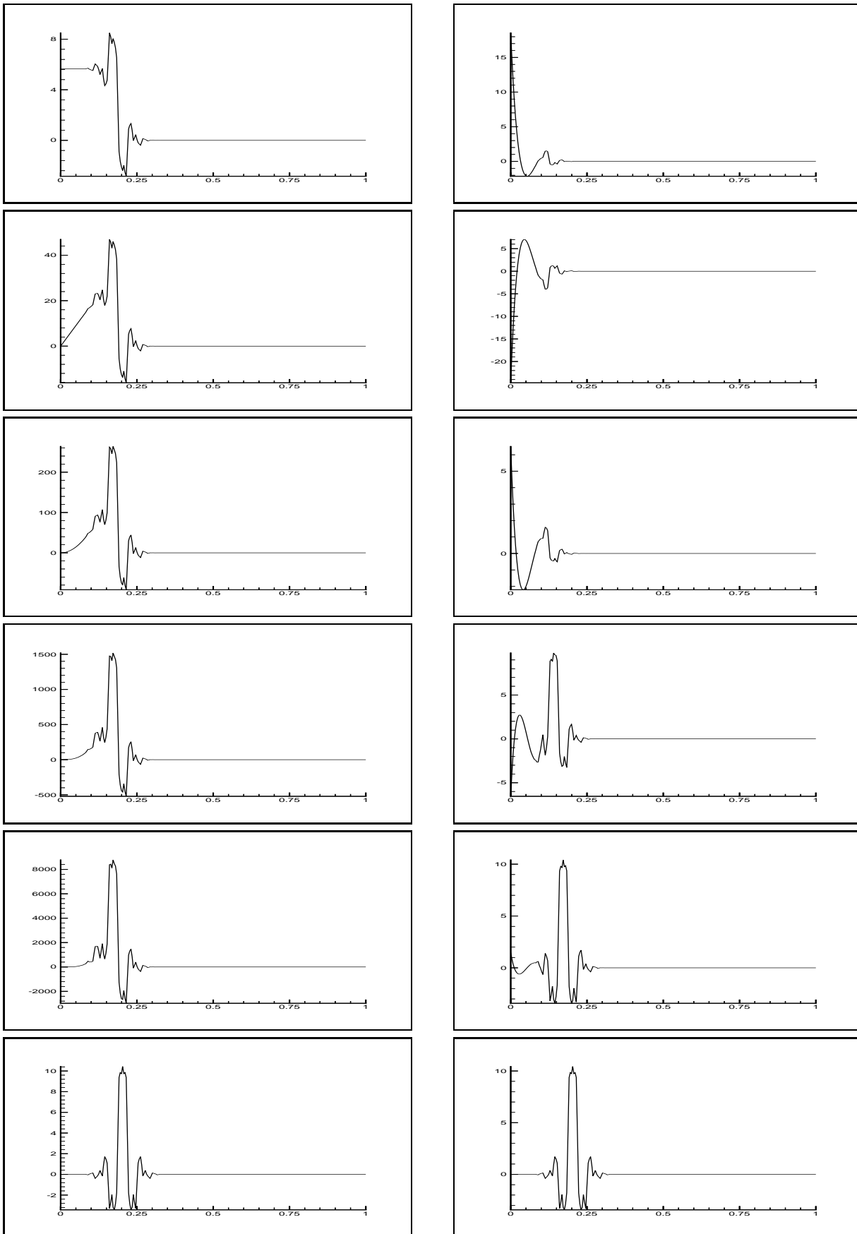
Figure 5.4.4: Dual generators \tilde{\phi}_{5,k} before and after biorthogonalization.
